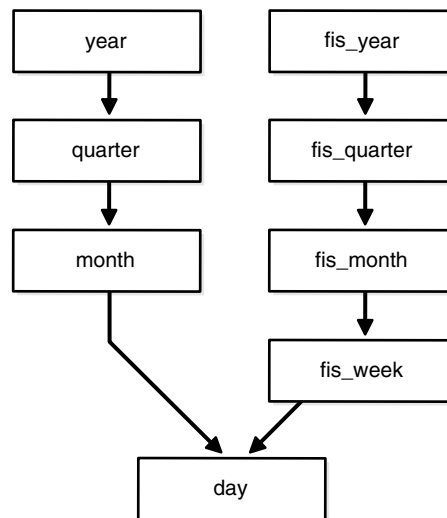
Figure 11-2 times_dim Dimension with Two Time Hierarchies
