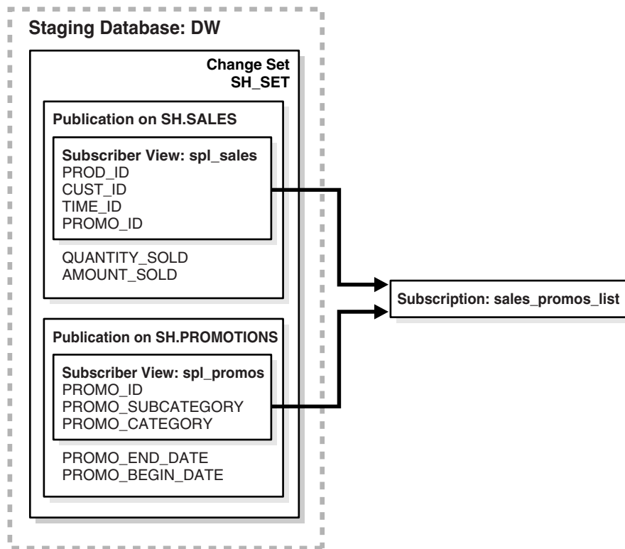
Figure 17–2 Subscriber Components in a Change Data Capture System
