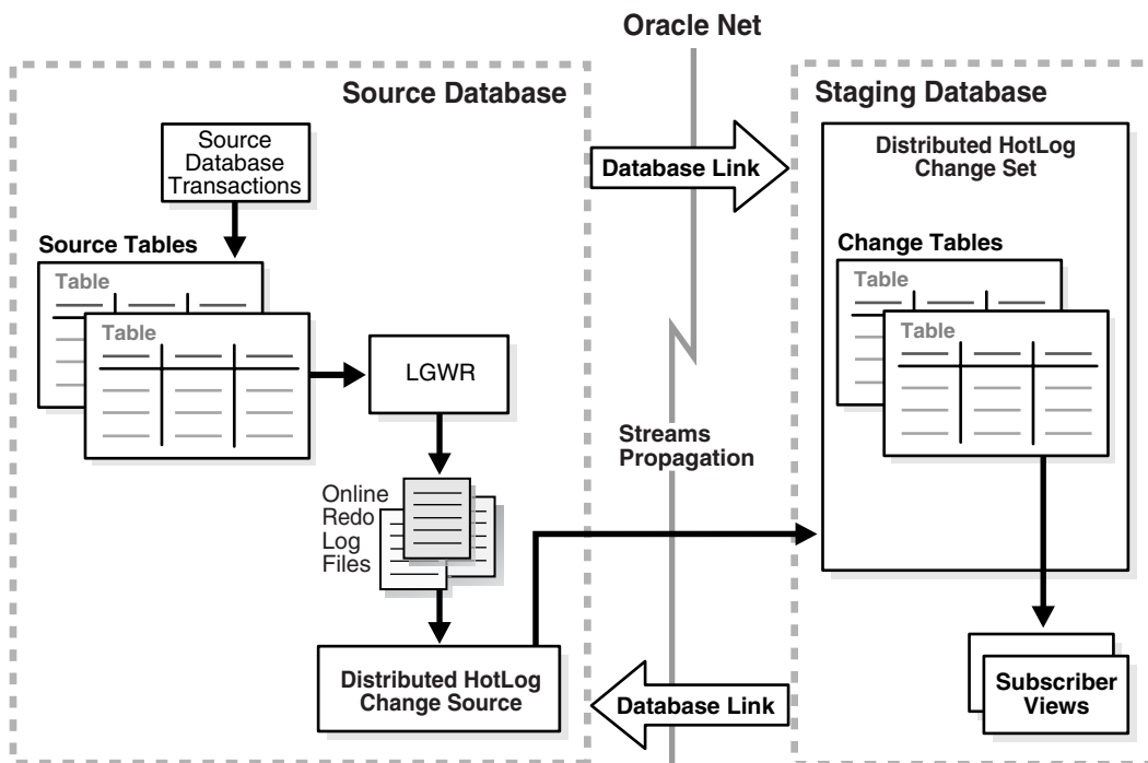
Figure 17-5 Asynchronous Distributed HotLog Configuration
