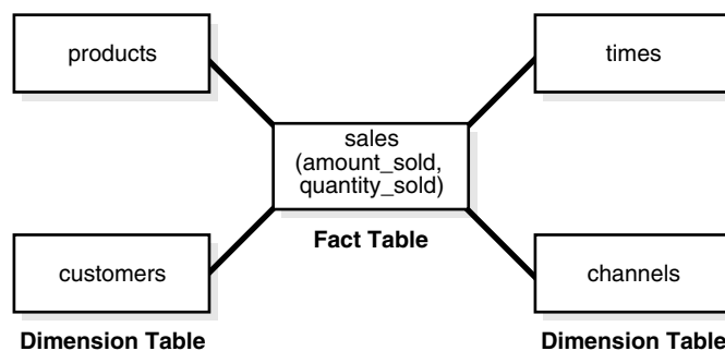
Figure 20-2 Star Schema
