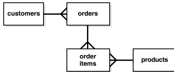
Figure 20-1 Third Normal Form Schema
