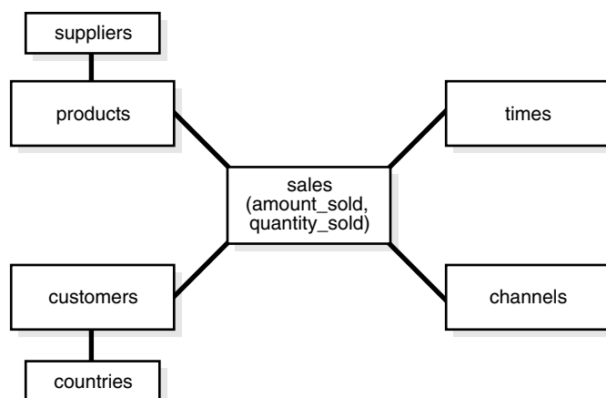
Figure 20–3 Snowflake Schema
