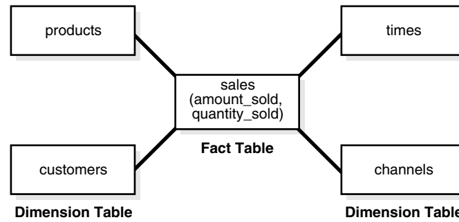
Figure 2-1 Star Schema
