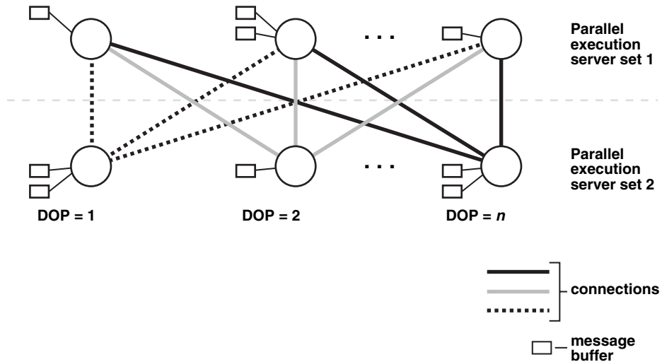
Figure 8–3 Parallel Execution Server Connections and Buffers
