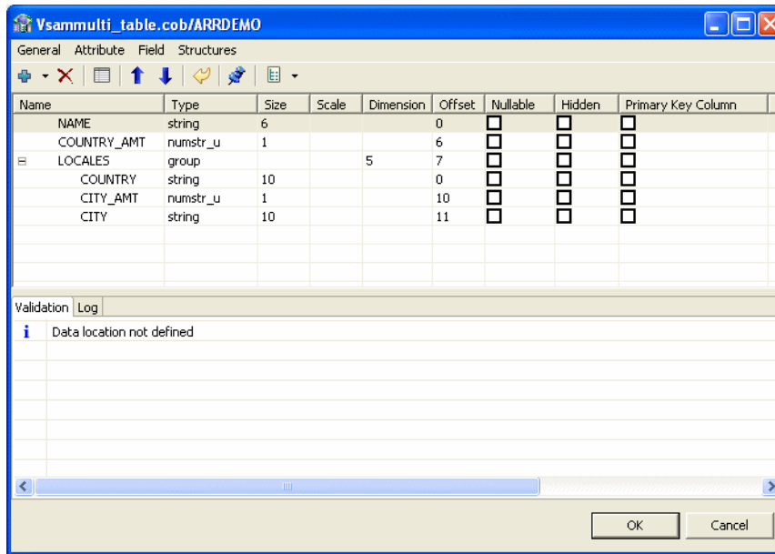
Figure 5–11 Field Manipulation Screen
