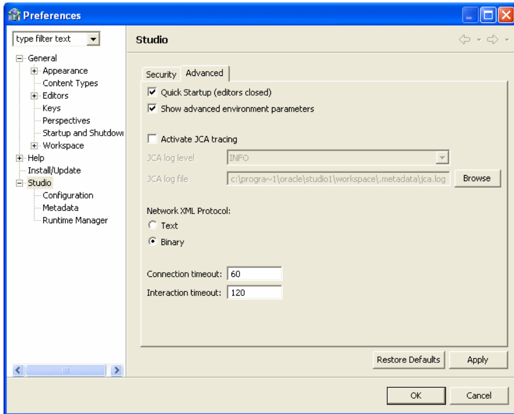
Figure 12–9 Studio Advanced Tab
