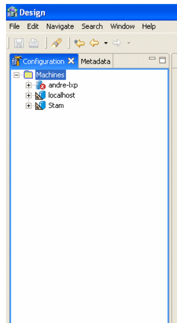
Figure 12–5 Configuration View
