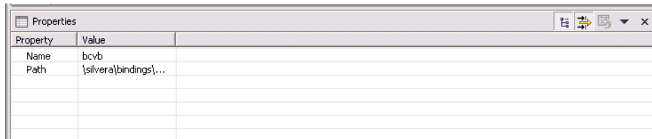
Figure 12–3 Properties View
