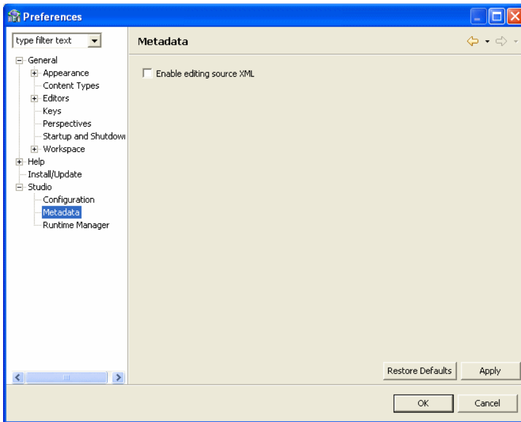
Figure 12–11 Metadata Preferences
