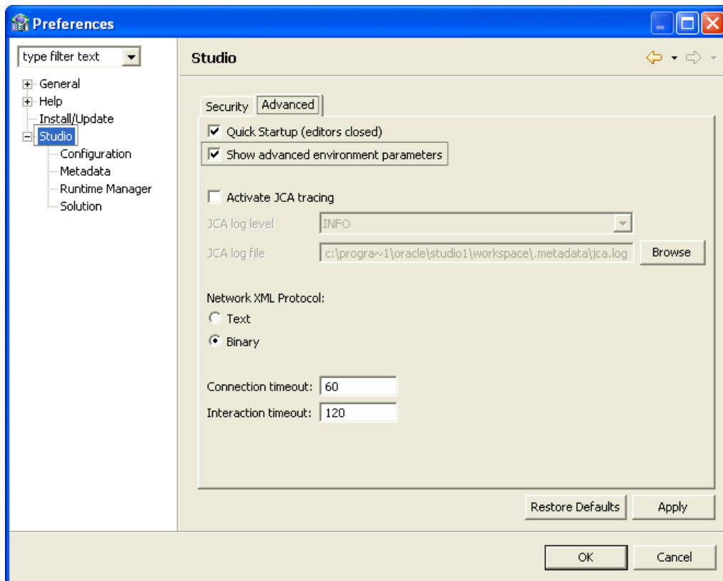
Figure 4–2 Studio Preferences
