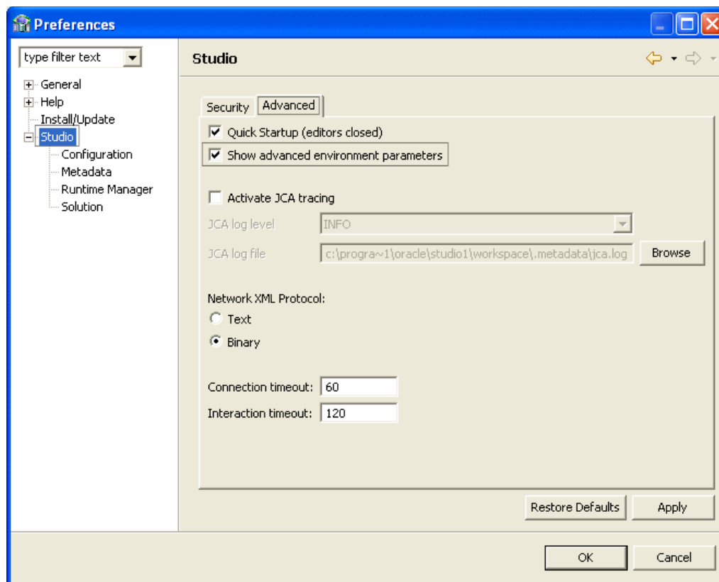
Figure 7-2 Studio Preferences
